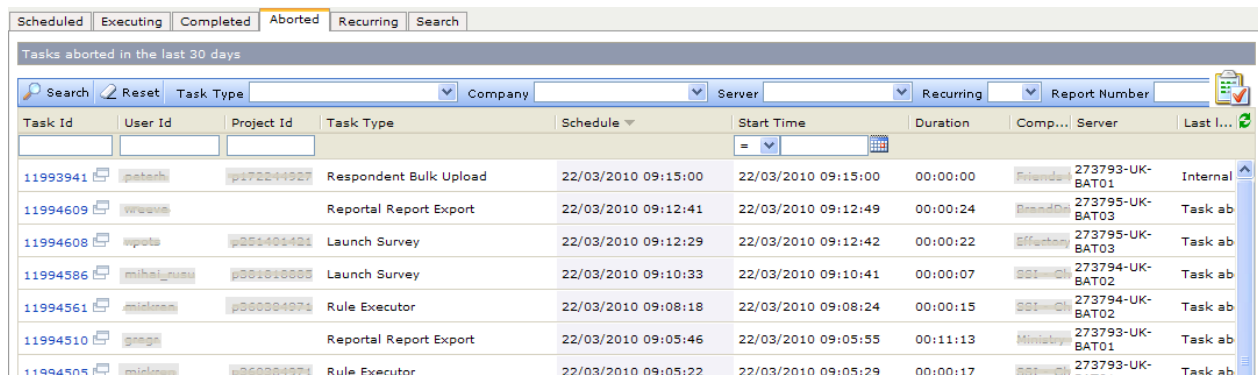
Figure 34 Example of the Error log
