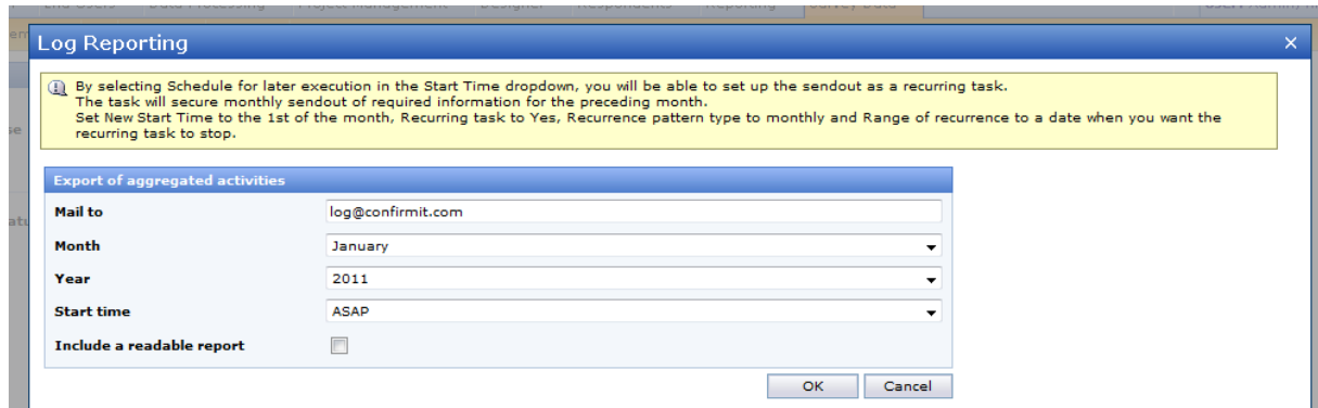
Figure 25 Log reporting
