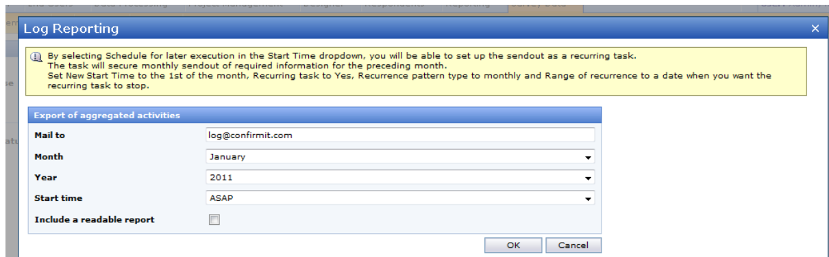
Figure 24 Log reporting
